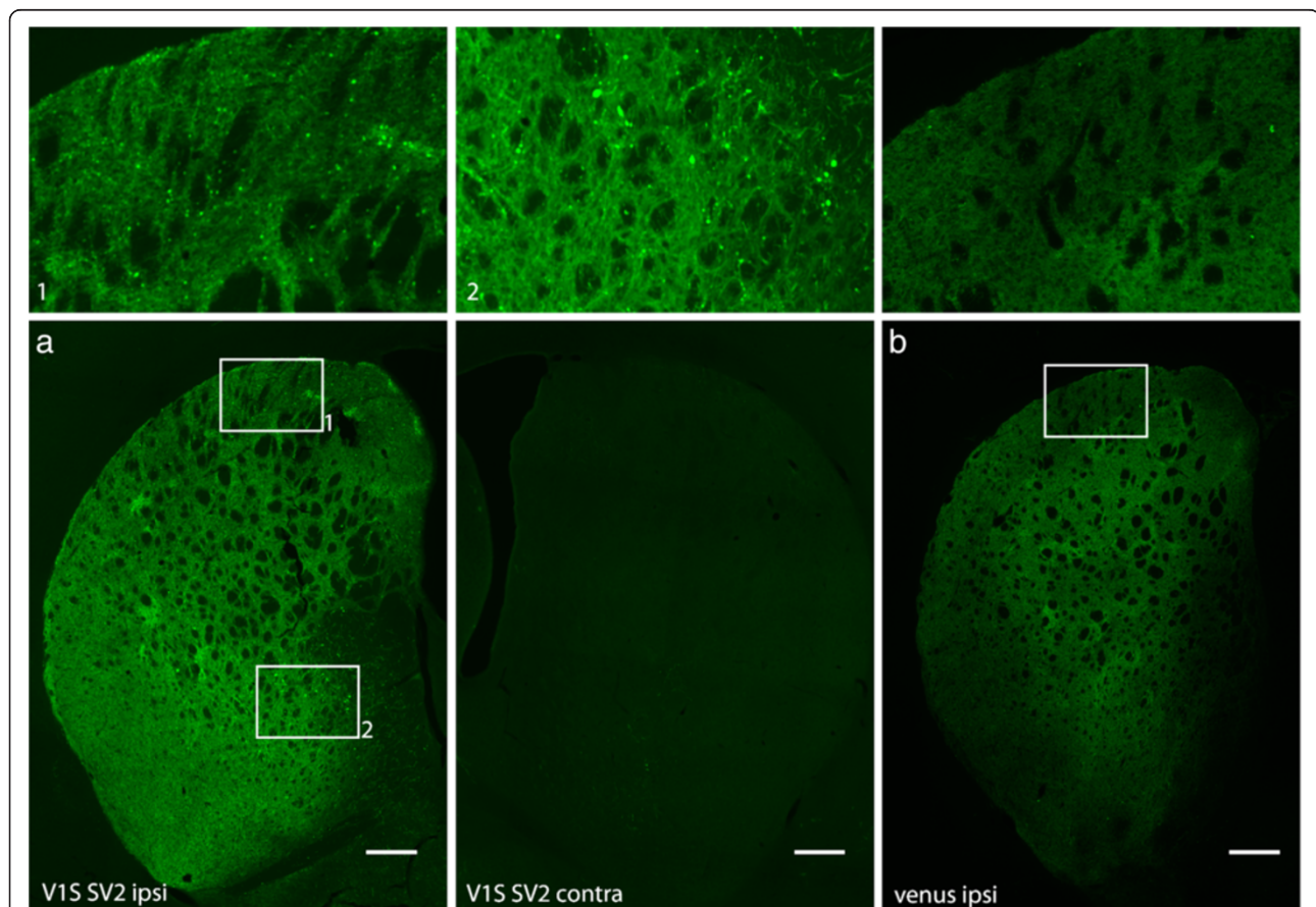
Figure 3 Detection of alpha synuclein oligomers in the striatum. The neuronal projections in the striatum of rats injected with AAV-V1S and AAV-SV2 in the SN were imaged for the presence of venusYFP fluorescence. Coronal sections from the striatum of rats injected into the SN were imaged under fluorescence microscope. VenusYFP is directly detected and localized to the striatum in animals injected with V1S and SV2, no fluorescence is detected contralateral (a). VenusYFP fluorescence is also detected in the striatum of rats injected with AAV-venus (b). Punctate fluorescence pattern is detected only in the striatum of animals injected with V1S and SV2 compared to the diffuse staining observed in animals injected with full length venusYFP (upper panel), suggestive for a possible accumulation of alpha synuclein within the striatum. Representative images are displayed. Scale bar 500 \mu m.
